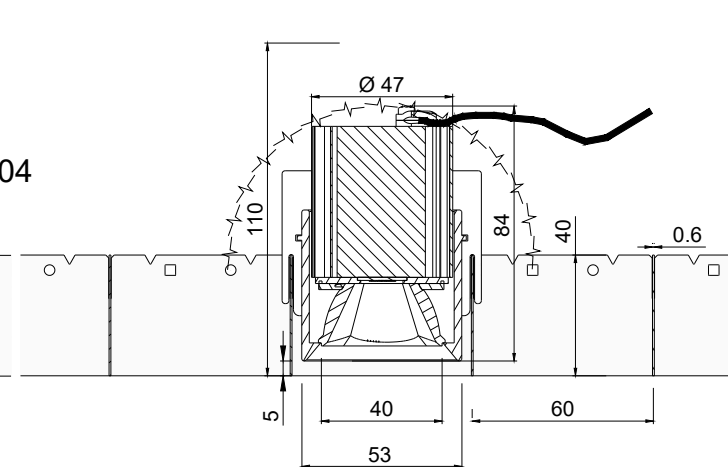
Cut view PUNTEO-J060 - S10 | LVK | Index "b" - 2 x 45°
