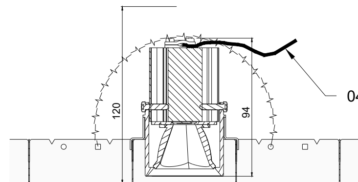
Cut view PUNTEO-J060 - S10 | LVK | Index "a" - 2 x 35°
