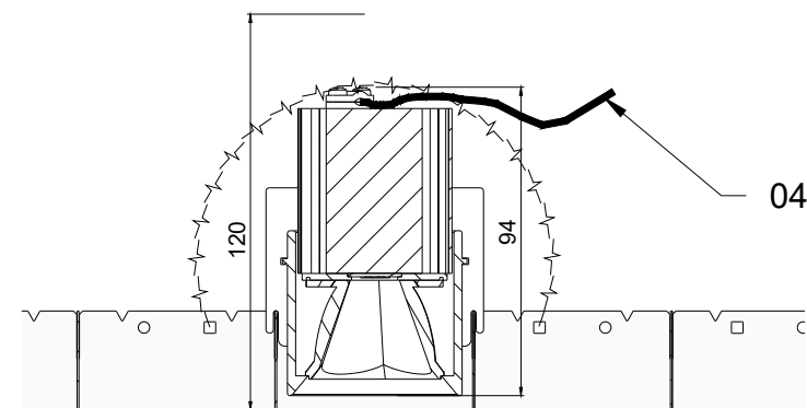
Cut view PUNTEO-J060 - S10 | LVK | Index "a" - 2 x 35°
