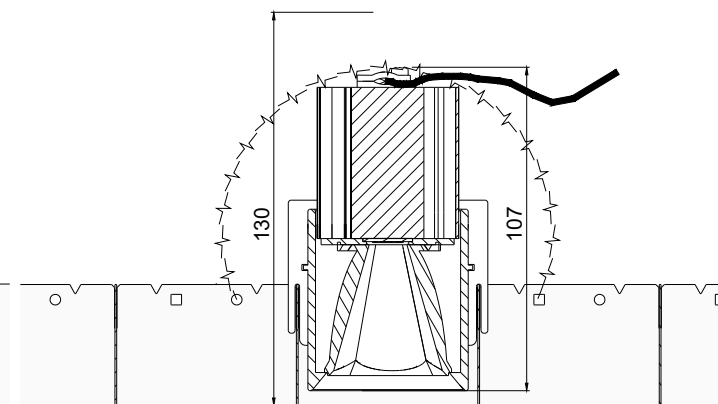
Cut view PUNTEO-J060 - S10 | LVK | Index "c" - 2 x 25°
