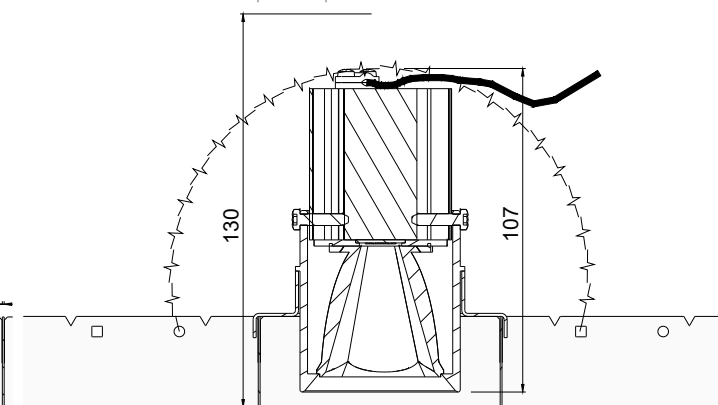
Cut view PUNTEO-J060 - S10 | LVK | Index "c" - 2 x 25°
